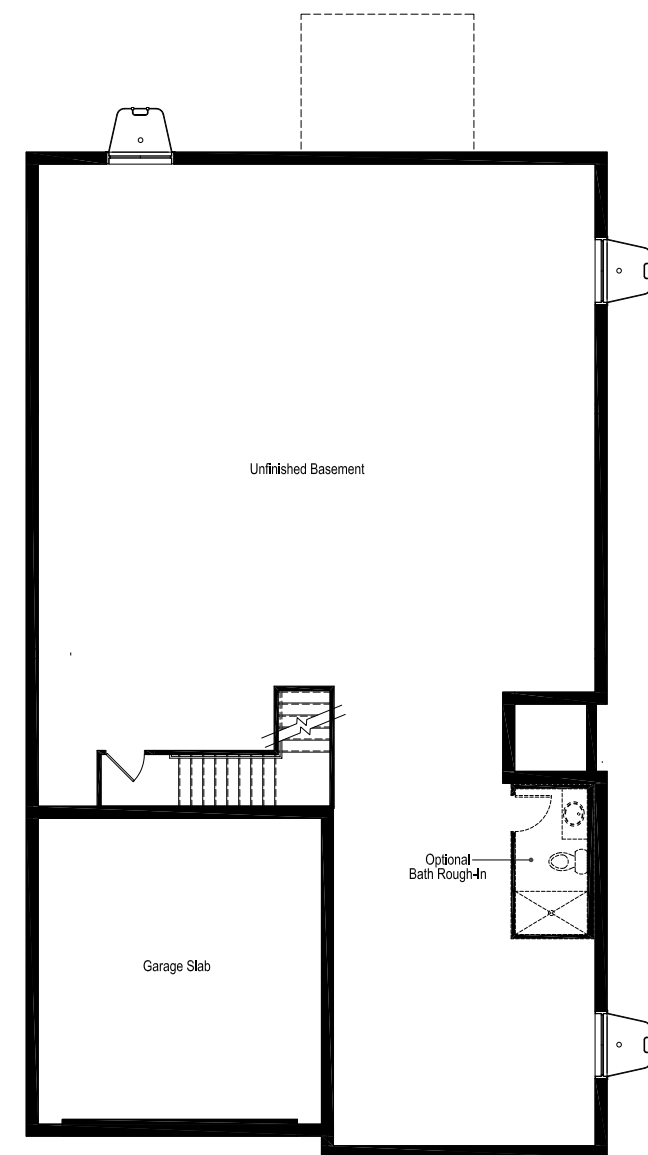
BASEMENT
