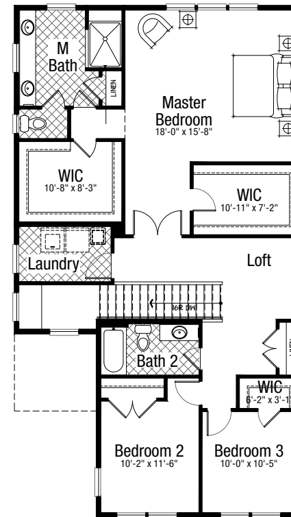
UPPER FLOOR
